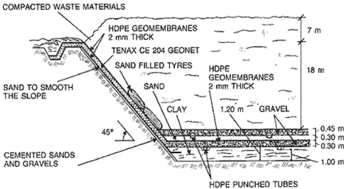
Fig. 2 - Schematic cross-section of the waste disposal
